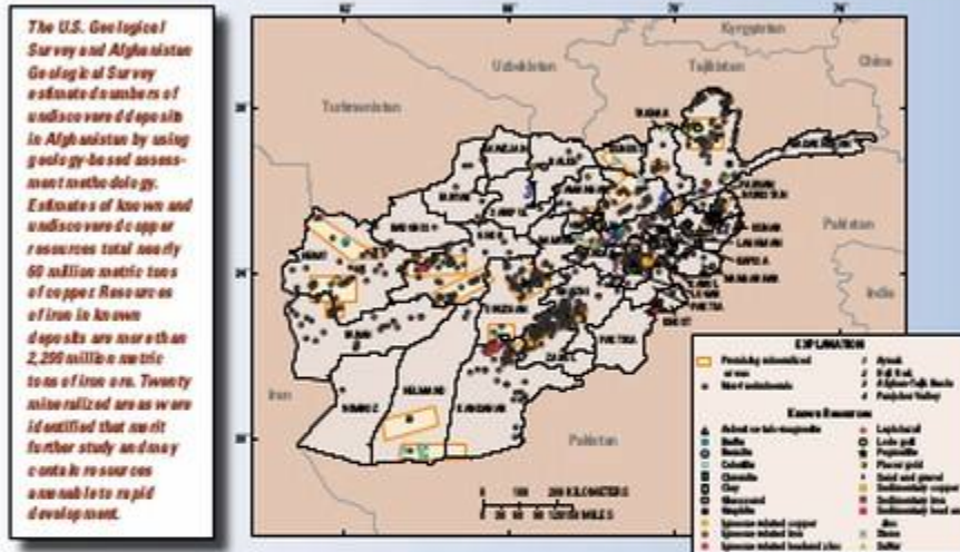
Figure 1. Map of Afghanistan showing mineralized areas recommended for further study (rectangular areas), known non-fuel mineral deposits and prospect potential (dots), and selected mineral deposits for which resources have been published in the past (various symbols).
